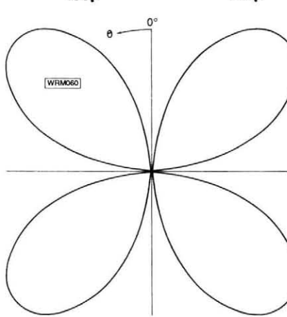
Fig. 7b: Coaxial loop
