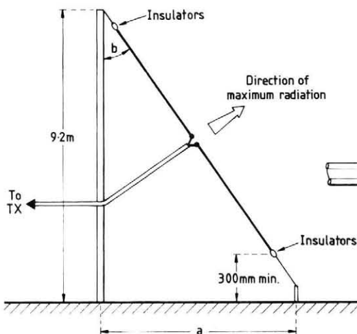
Fig. 1, for single band operation doubled-up 75Ω balanced twin can be used, Fig. 2.
