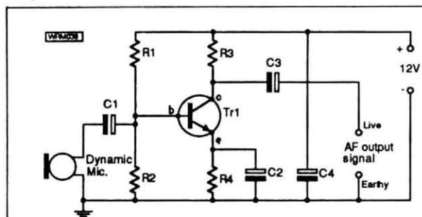
Fig. 14.1: A microphone amplifier
