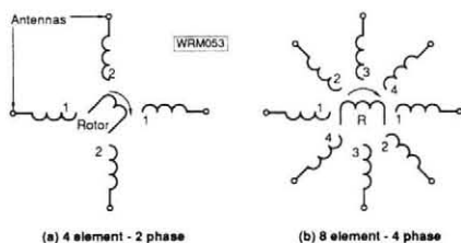
Fig. 6: Plan view of Adcock arrays with goniometer. Stator coils are connected diametrically across centre, as 1 to 1, 2 to 2
