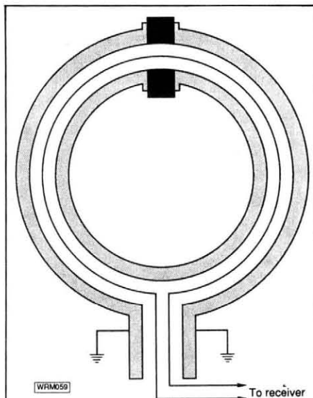
Fig. 1a: A screened loop antenna
