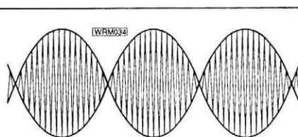
Fig. 14.3: Balanced modulator output waveform for single tone a.f. input
