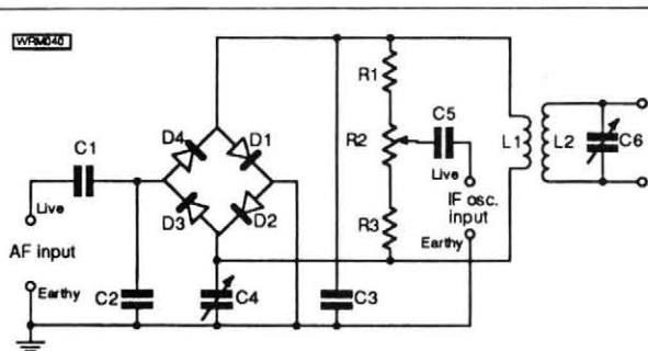
Fig. 14.2: A balanced modulator
