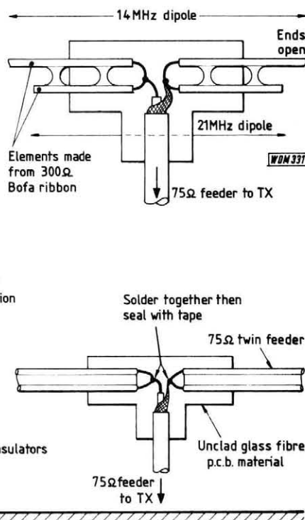
Fig. 1: Dual-band dipole using 300Ω Bofa ribbon
