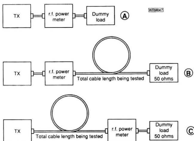
Fig. 1: Checking a length of coaxial cable for power loss
